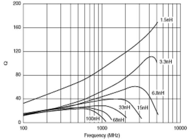
Q-Frequency Characteristics
