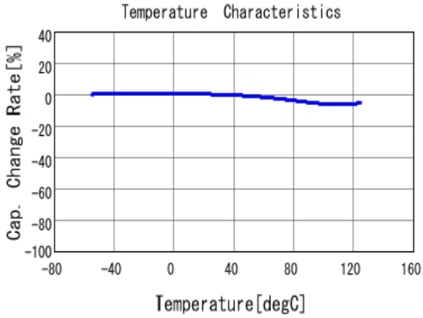
■ GRM033R71A152KA01 C-Temp. capchange, DCO. 0V, AC1.0V rm
