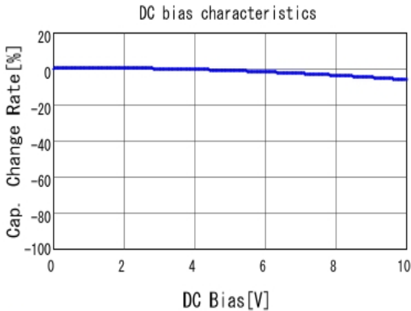
■ GRM033R71A152KA01 C-DC bias capchange, 25.0degC, AC1.
