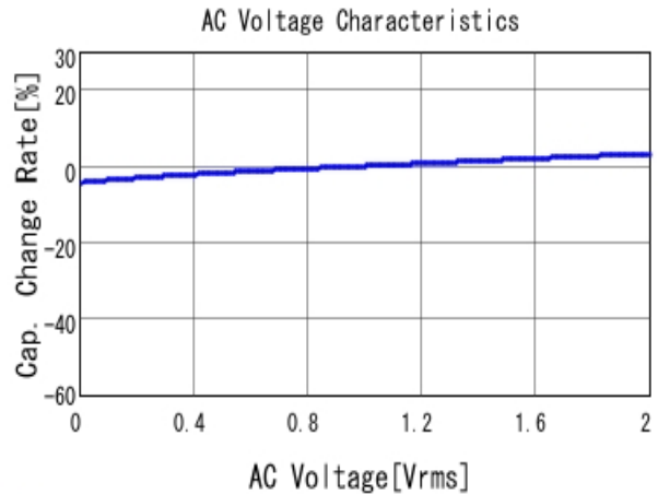
■ GRM033R71A152KA01 C-AC Voltage capchange, DCOV, 25.0d
