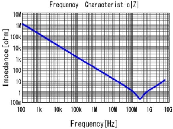
■ GRM033R71A152KA01 |Z| DCOV, 25degC
