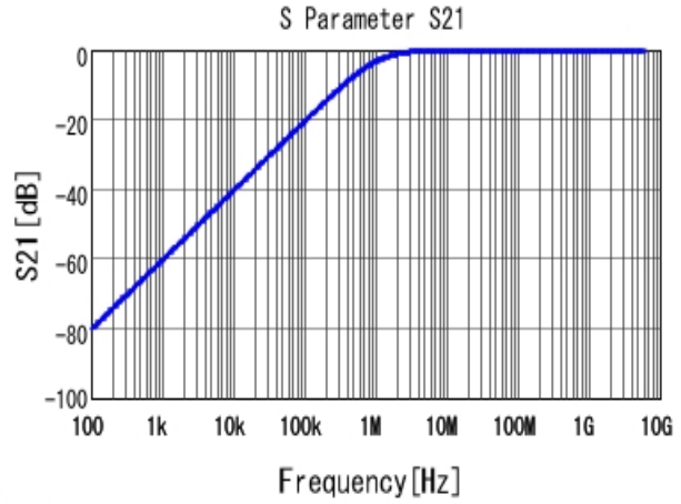
■ GRM033R71A152KA01 S21 DCOV, 25degC
