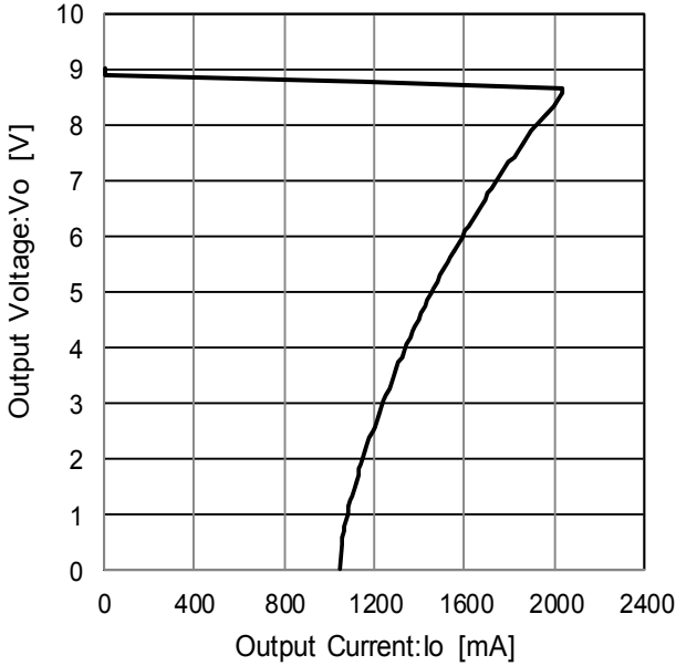
Figure 63. Load Regulation
