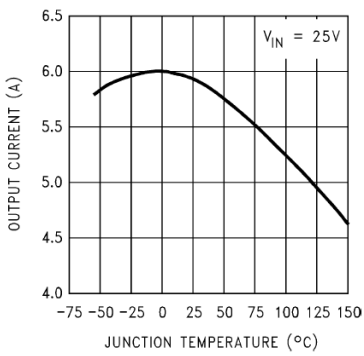
Current Limit
