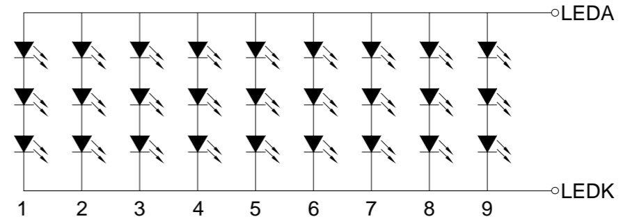
LED Diagram Circuit
