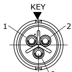
WIRING END W6382-3PG-P-5XX
