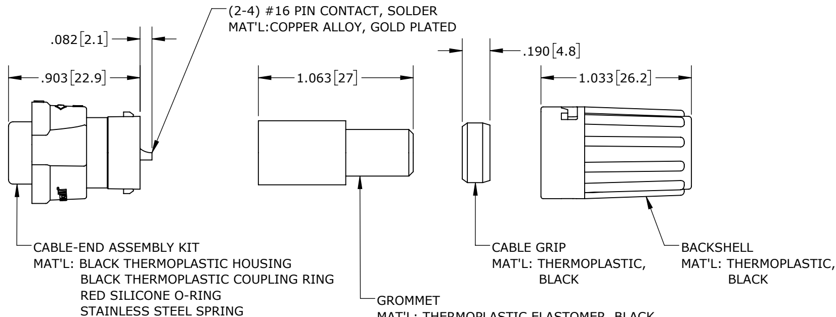
SHOWN ASSEMBLED KIT ASSY: W6382-2PG-P-5XX SHOWN
