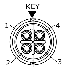
WIRING END W6382-4PG-P-5XX
