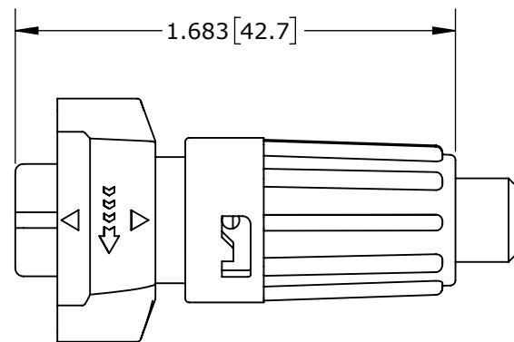
SHOWN ASSEMBLED KIT ASSY: W6382-2PG-P-5XX SHOWN
