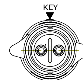
WIRING END ASSY: W6382-2PG-P-5XX SHOWN WITHOUT HARDWARE
