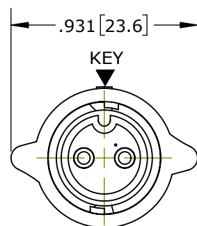
MATING FACE ASSY: W6382-2PG-P-5XX SHOWN
