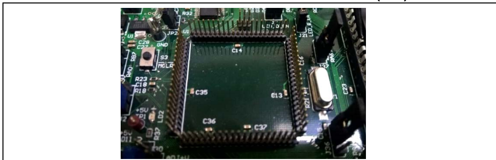
FIGURE 2-1: 84-PIN HEADER FOR PLUG-IN-MODULE (PIM)
