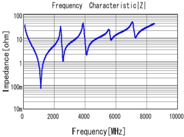
■ GQM2195C2E470JB12 |Z| DCOV, 25degC
