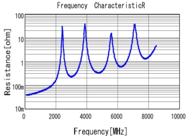
■ GQM2195C2E470JB12 R DCOV, 25degC
