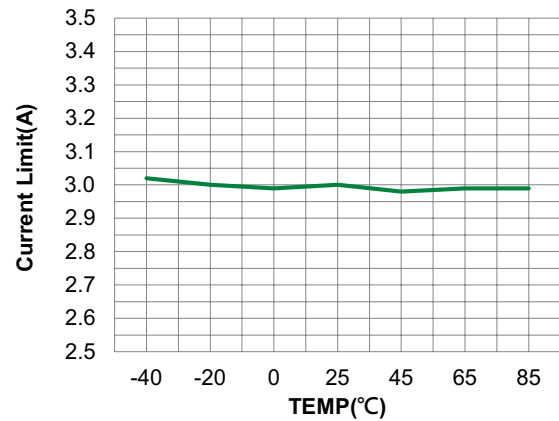
Figure 2. Programmable Current Limit ( R_{LIMIT}=3.3K )
