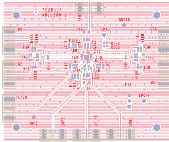
Figure 103. Evaluation Board Top Layer
