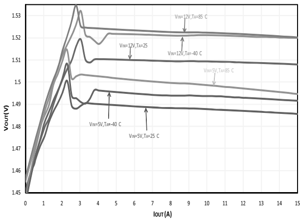
Load Regulation vs. Temperature - P-Save (V DD = 5 V, V OUT T = 1.5 V, SiC401B)
