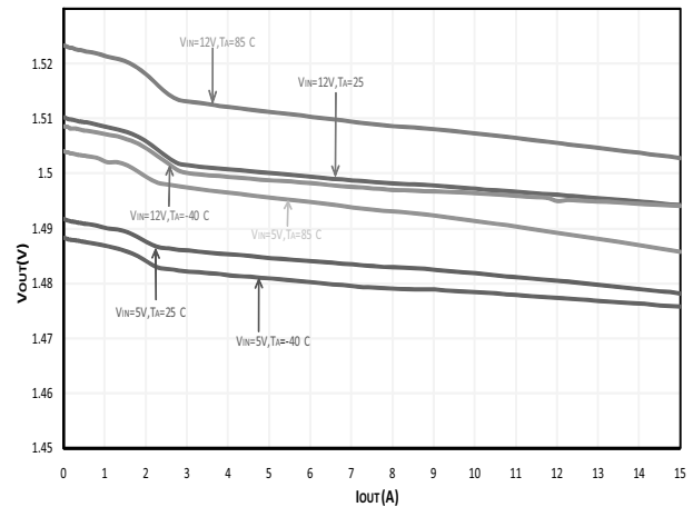
Load Regulation vs. Temperature - FCM (V DD = 3.3 V, V OUT T = 1.5 V, SiC401B)
