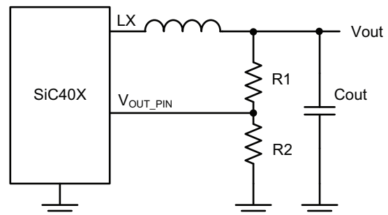
Fig. 18 - Resistor Divider Network allows 4.5 V at the V_{\text{OUT}} Pin
