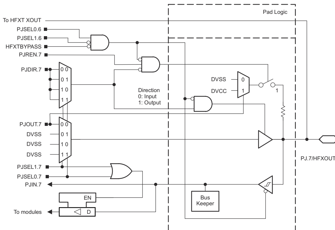
Figure 9-24. Port PJ (PJ.7) Diagram
