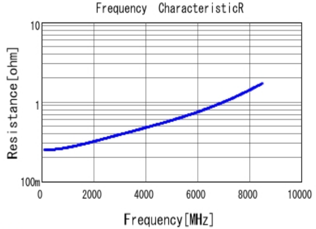
■ GRM0335C1H3R3CA01 R DC0V, 25degC
