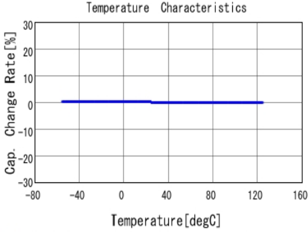
■ GRM0335C1H3R3CA01 C-Temp. capchange, DCOV, AC1Vrms
