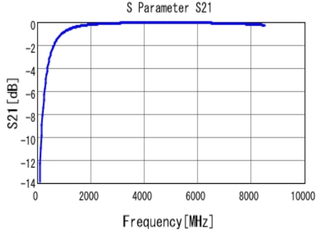
■ GRM0335C1H3R3CA01 S21 DCOV, 25degC
