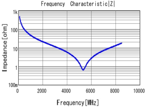
■ GRM0335C1H3R3CA01 |Z| DC0V, 25degC
