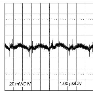
Figure 14. Output Ripple
