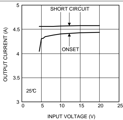
Figure 17. Current Limit 1.8\text{ V}_{OUT} at 25^\circ\text{C}
