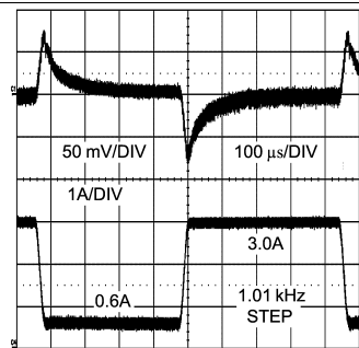
Figure 15. Transient Response
