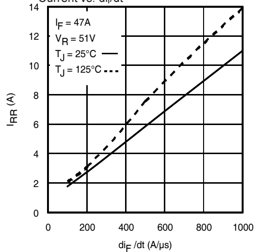
Fig 18. - Typical Recovery Current vs. di/dt
