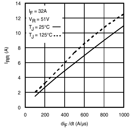
Fig 17. - Typical Recovery
