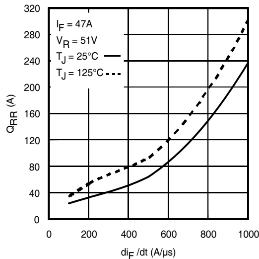
Fig 20. - Typical Stored Charge vs. di/dt
