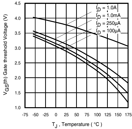
Fig 16. Threshold Voltage vs. Temperature Current vs. di/dt
