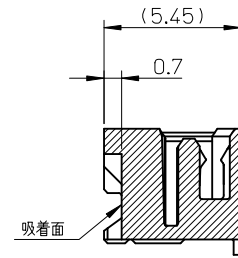
SECTION Y-Y
