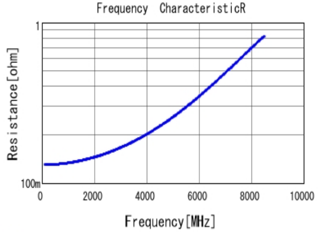
GJM1555C1H3R6CB01 R DC0V, 25degC
