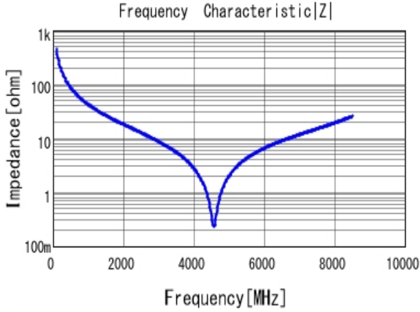
GJM1555C1H3R6CB01 |Z| DC0V, 25degC
