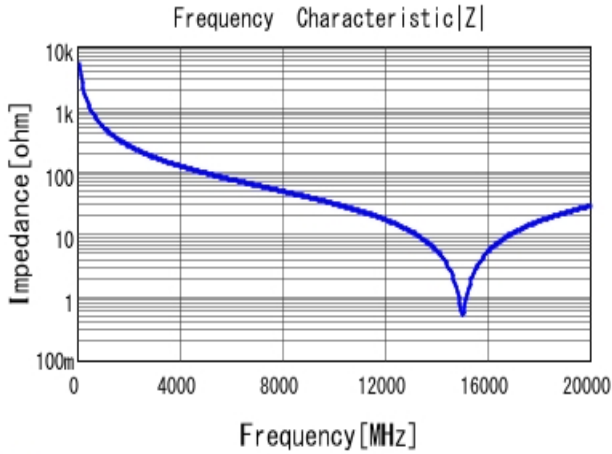
GJM1555C1HR30WB01 |Z| DC0V, 25degC
