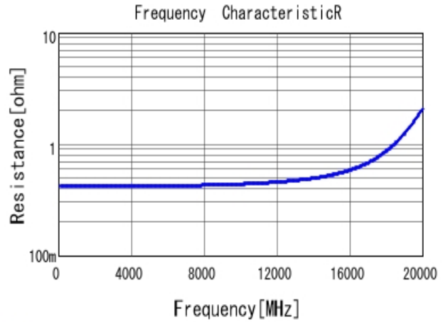
GJM1555C1HR30WB01 R DC0V, 25degC
