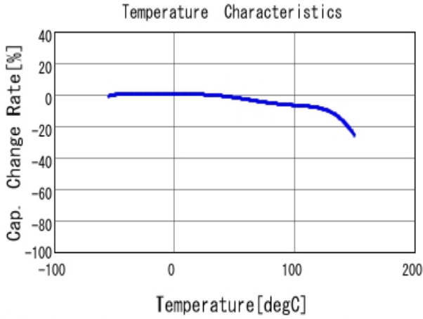
■ GCM155L81C473KA37 C-Temp. capchange, DCO. 0V, AC1.0V rm
