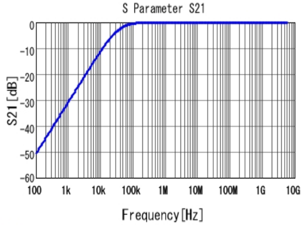
■ GCM155L81C473KA37 S21 DCOV, 25degC
