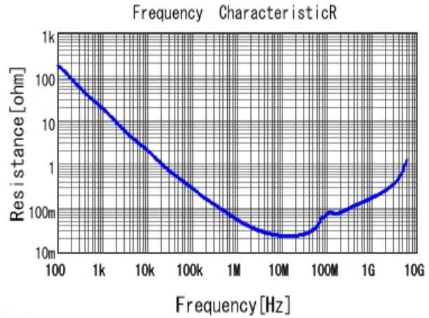
GCM155L81C473KA37 R DCOV, 25degC
