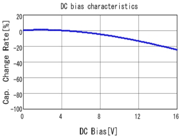
GCM155L81C473KA37 C-DC bias capchange, 25.0degC, AC1.
