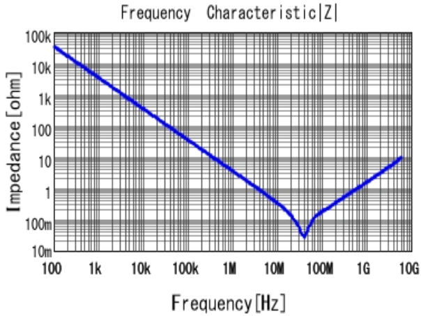
GCM155L81C473KA37 |Z| DCOV, 25degC
