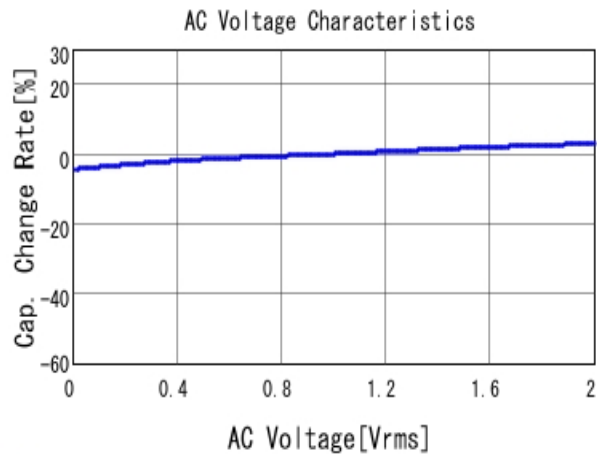
GCM155L81C473KA37 C-AC Voltage capchange, DCOV, 25.0d
