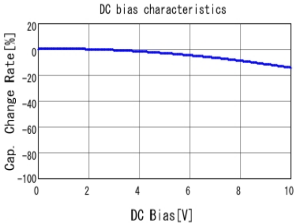
■ GRM31MR71A225KA01 C-DC bias capchange, 25.0degC, AC1.
