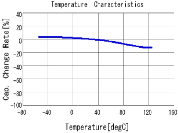
■ GRM31MR71A225KA01 C-Temp. capchange, DC0.0V, AC1.0V r m
