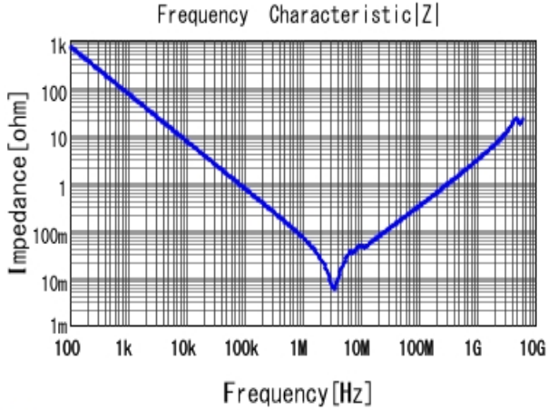
■ GRM31MR71A225KA01 |Z| DCOV, 25degC
