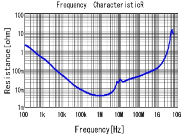
■ GRM31MR71A225KA01 R DCOV, 25degC
