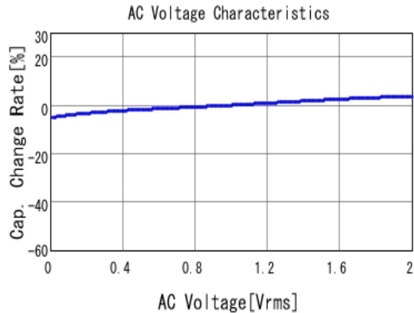
■ GRM31MR71A225KA01 C-AC Voltage capchange, DCOV, 25.0d
