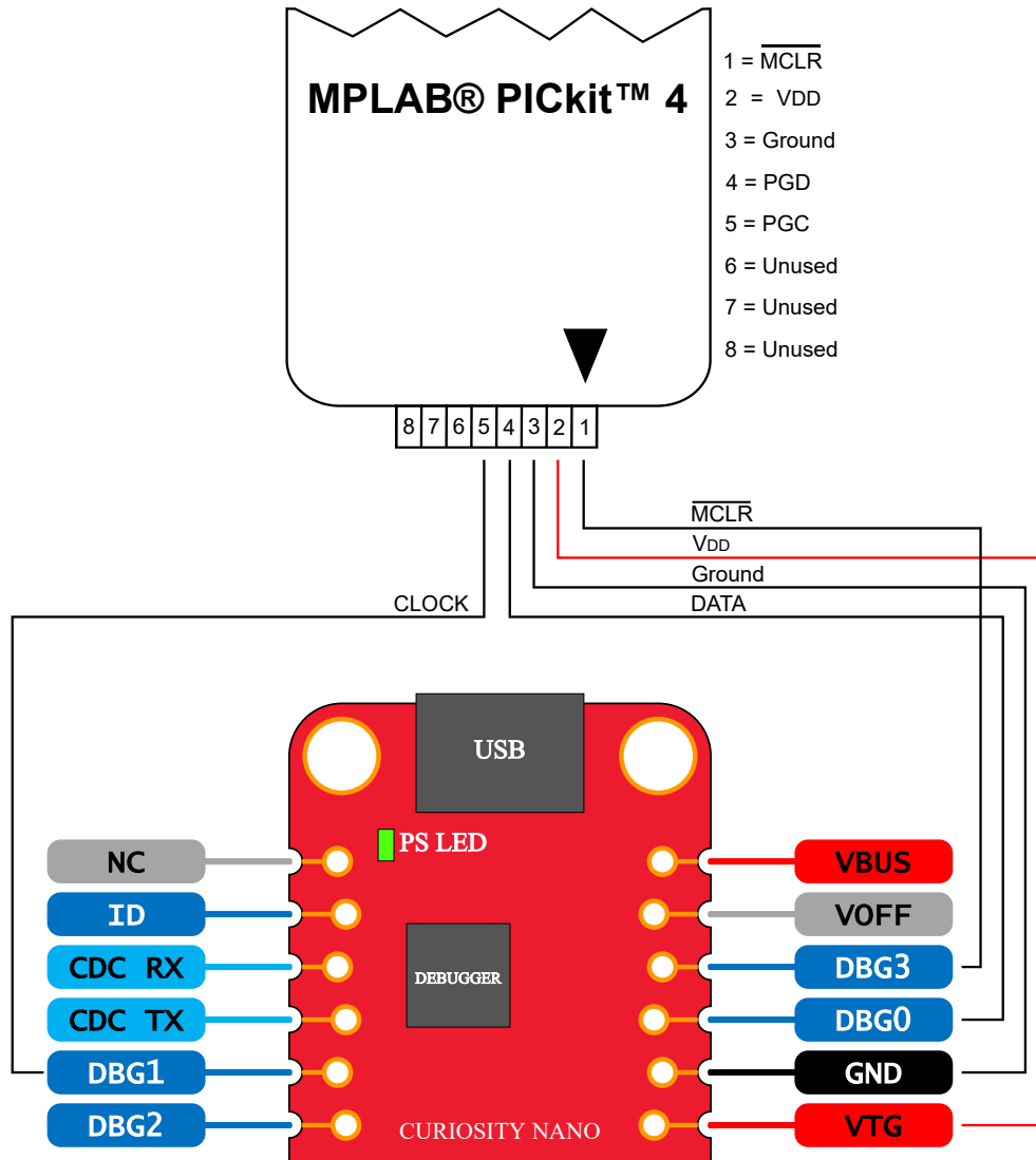
Figure 7-5. Connecting the MPLAB PICKit™ 4 In-Circuit Debugger/Programmer to PIC16F18446 Curiosity Nano
