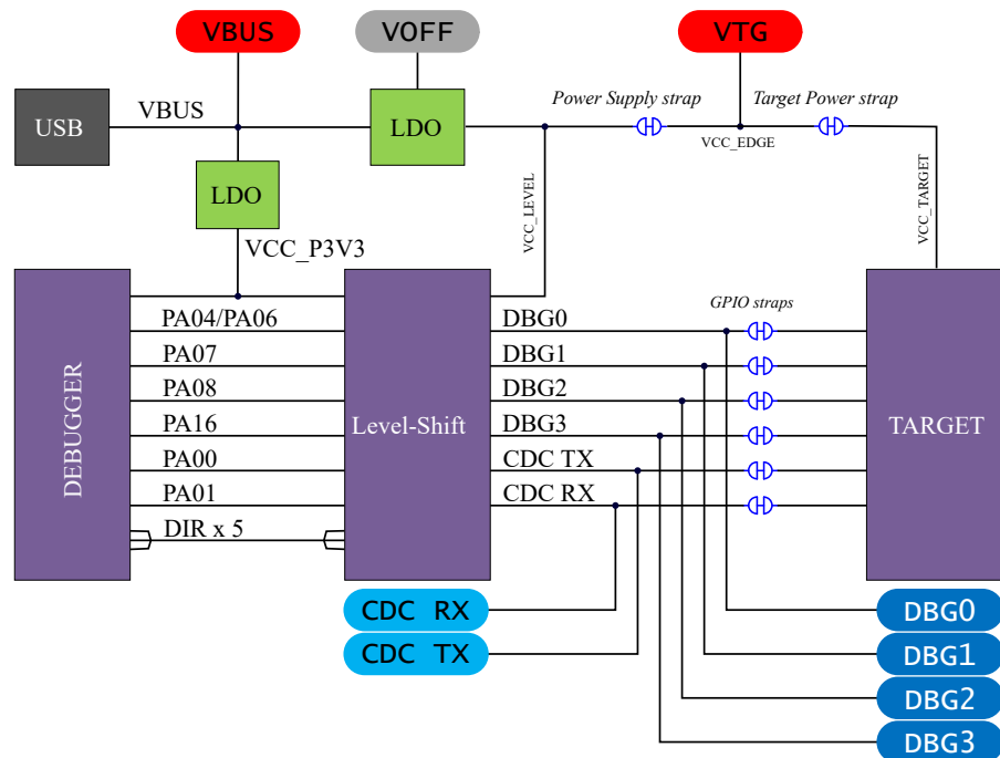
Figure 3-6. On-Board Debugger Connections to the PIC16F18446
