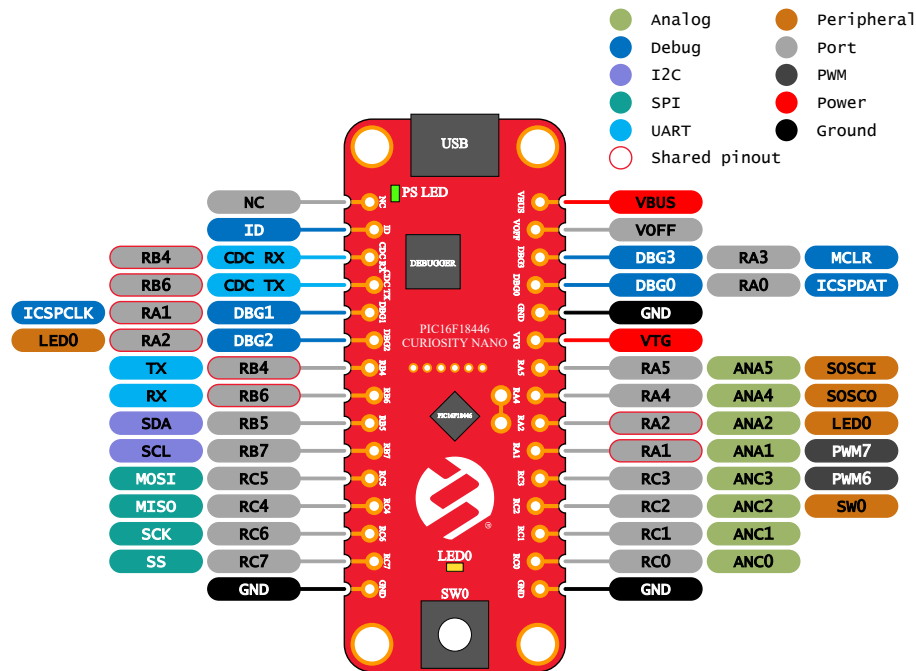
Figure 4-1. PIC16F18446 Curiosity Nano Pinout
