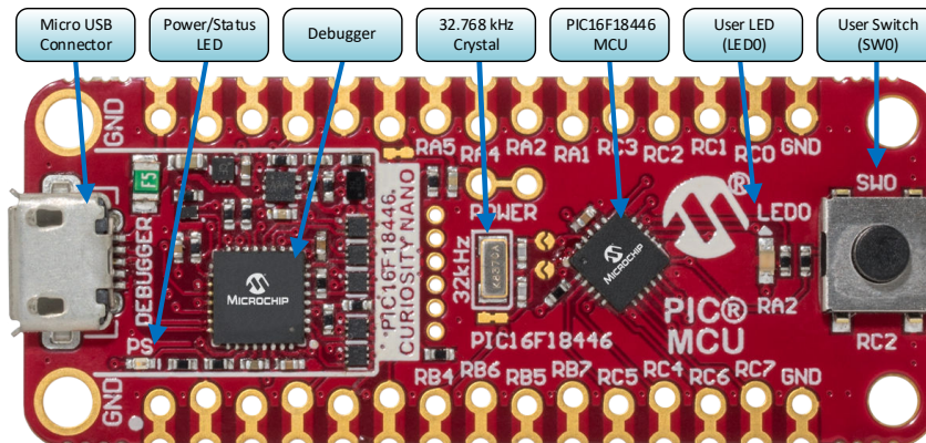
Figure 1-1. PIC16F18446 Curiosity Nano Evaluation Kit Overview
