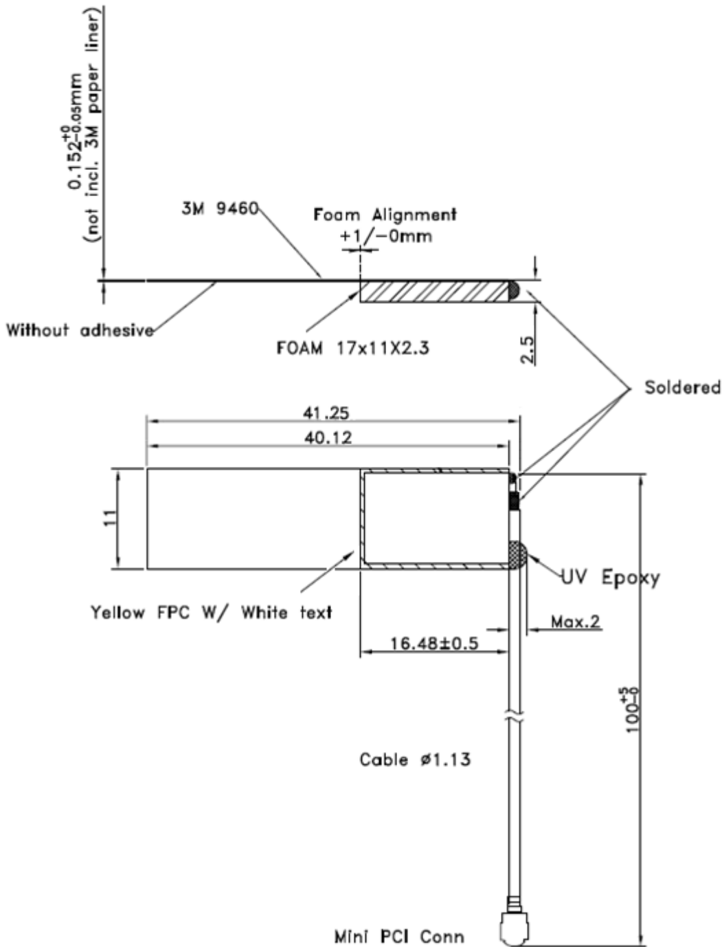
Figure 1: FlexPIFA mechanical drawing of 001-0014 and 001-0022
