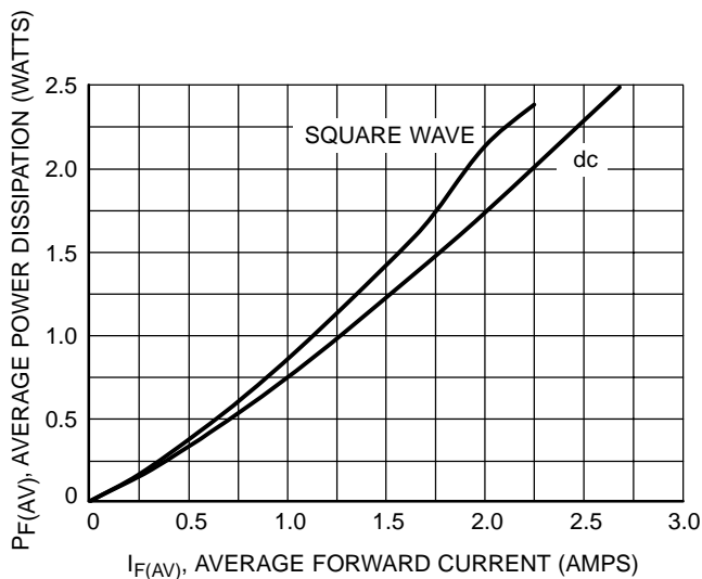
Figure 6. Power Dissipation
