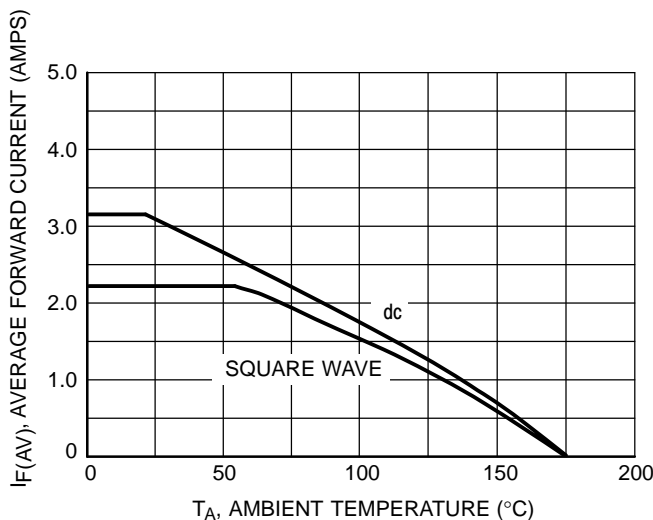
Figure 5. Current Derating
