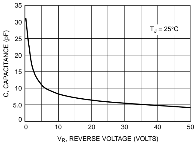
Figure 8. Maximum Capacitance
