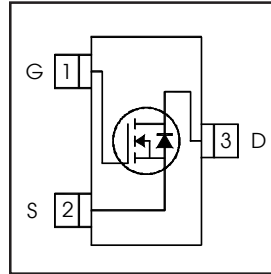
Micro3™ (SOT-23) IRLML2030TRPbF
