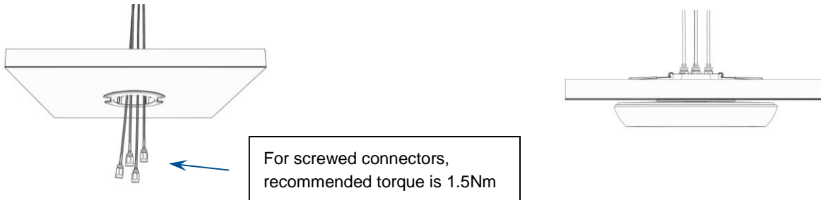
Figure 5: Installation of the Antenna
