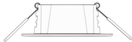
Figure 3: Upper mounting position 16-40mm / 5/8"-1 1/2" ceiling thickness
