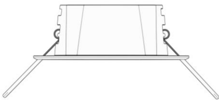
Figure 2: Lower mounting position 3-16mm / 0.1-5/8" ceiling thickness (pre mounted)
