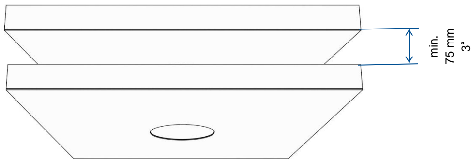
Figure 1: Clearance between the ceilings: Clearance between the solid and the suspended-ceiling shall be > 75mm / 3"
