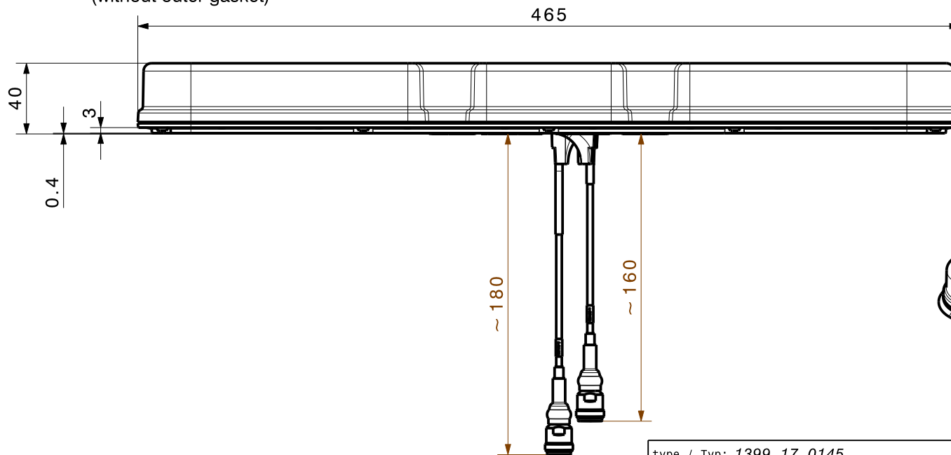
Side view (without outer gasket)
