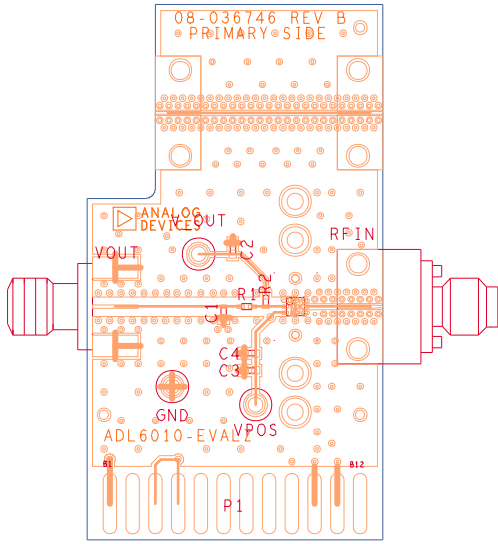
Figure 48. ADL6010 Evaluation Board Layout, Top Side
