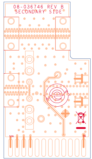
Figure 49. ADL6010 Evaluation Board Layout, Bottom Side
