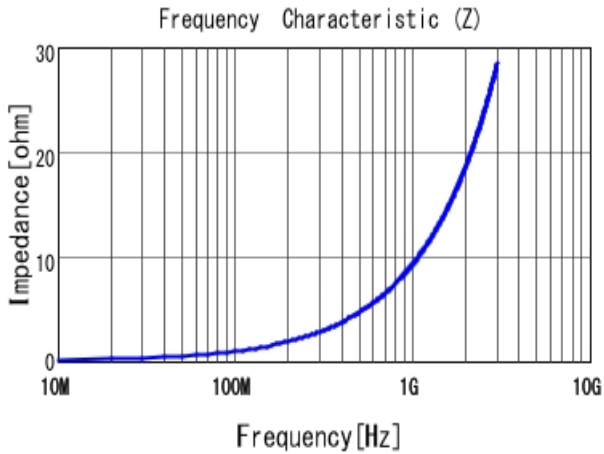
■ LQP15MN1N5W02 |Z|
