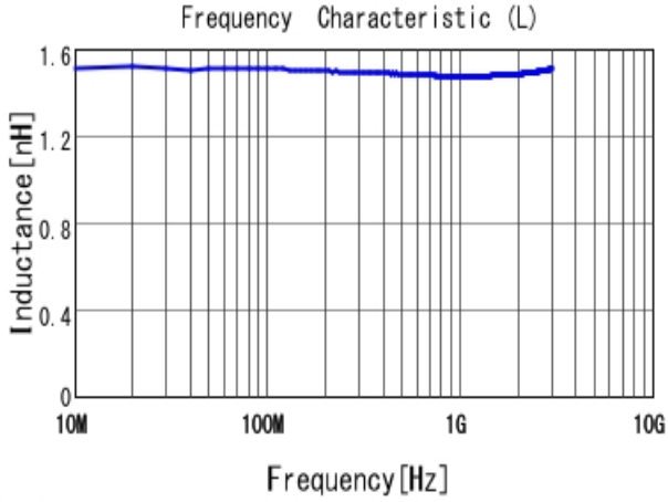
■ LQP15MN1N5W02 L
