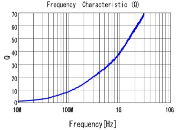
■ LQP15MN1N5W02 Q
