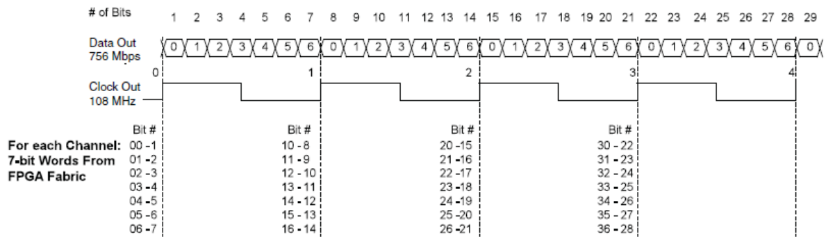
Figure 5.5. DDRX71, DDRX141 Video Timing Waveforms
