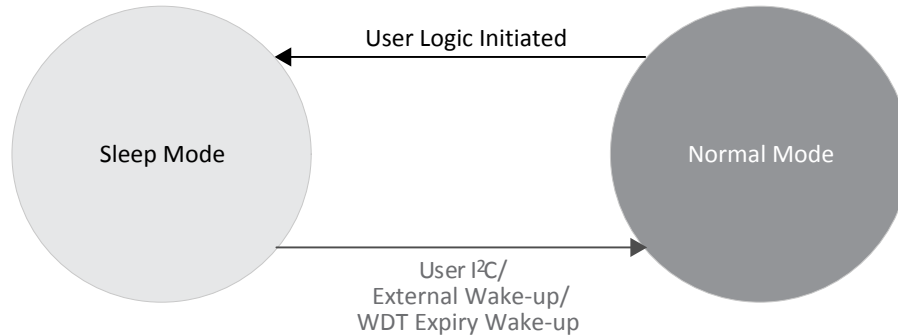
Figure 4.4. CrossLink PMU State Machine
