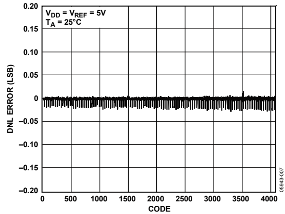
Figure 8. DNL AD5624
