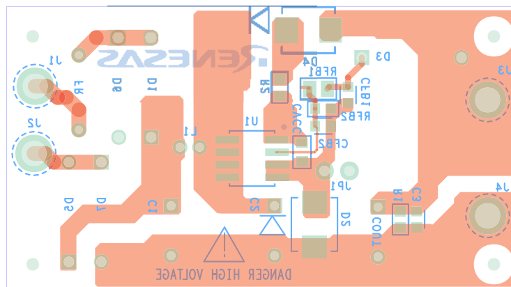
Figure 6. Bottom Layer
