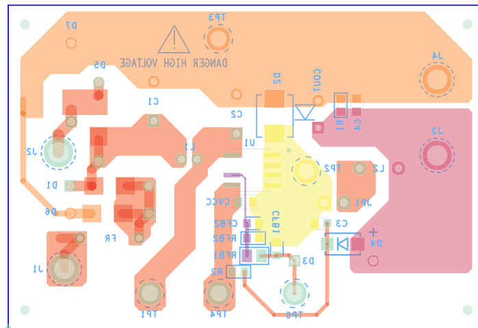
Figure 6. Bottom Layer
