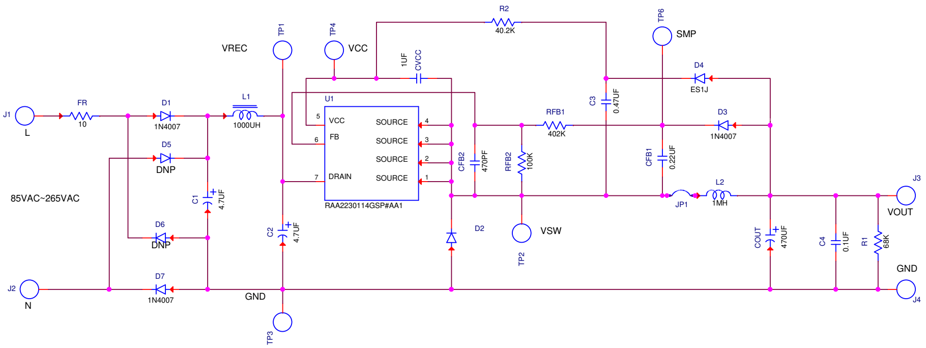
Figure 4. RTKA223011DE0020BU Schematic
