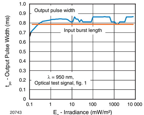
Fig. 2 - Pulse Length and Sensitivity in Dark Ambient
