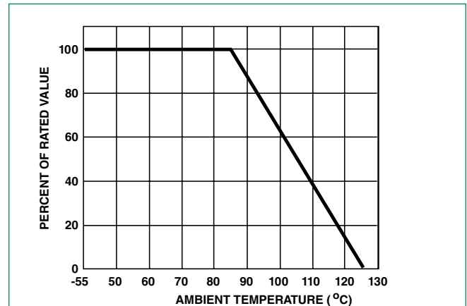
Figure 2. Current, Energy, Power Derating Curve
