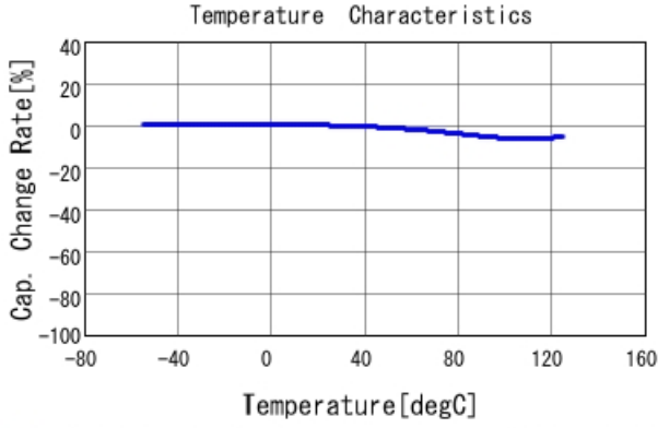
■ GRM033R71H681KA12 C-Temp. capchange, DCO. 0V, AC1. 0Vrm
