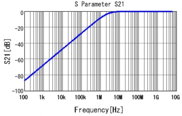
■ GRM033R71H681KA12 S21 DCOV, 25degC
