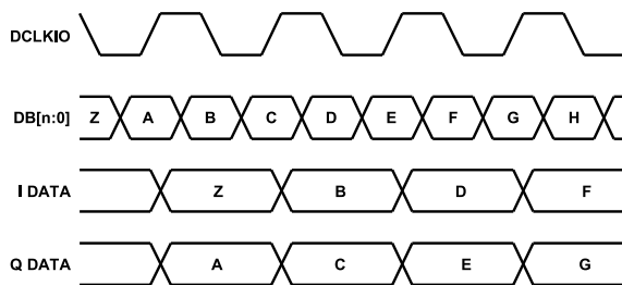
Figure 90. Timing Diagram with IFIRST = 0, IRISING = 1
