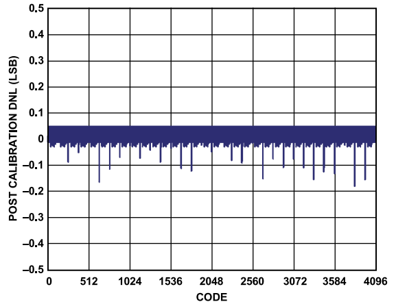
Figure 22. AD9116 Postcalibration DNL at 3.3 V, 20 mA
