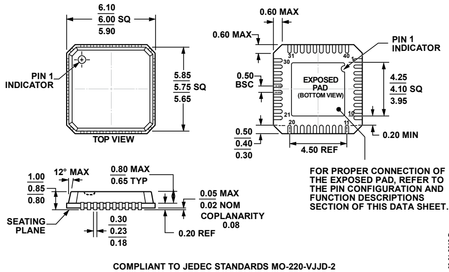
Figure 112. 40-Lead Lead Frame Chip Scale Package [LFCSP] 6 mm × 6 mm and 0.85 mm Package Height (CP-40-1) Dimensions shown in millimeters
