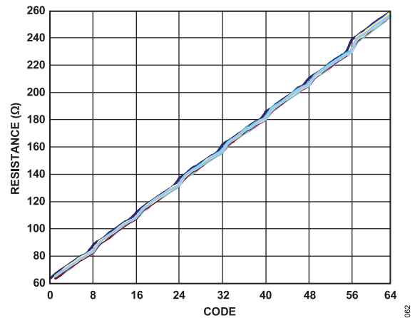
Figure 102. Typical CML Resistor Value vs. Register Code
