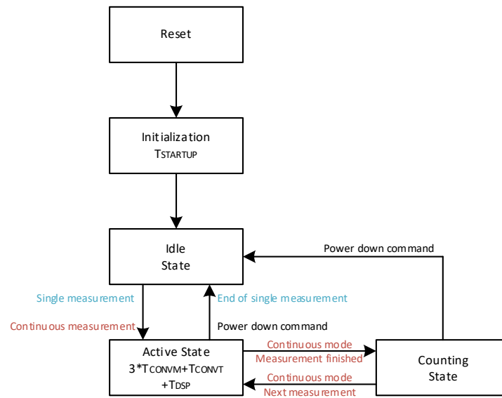
Figure 13: Sequence flowchart
