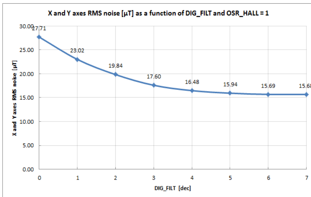
Figure 20: version 011 - XY axis RMS noise (typ)
