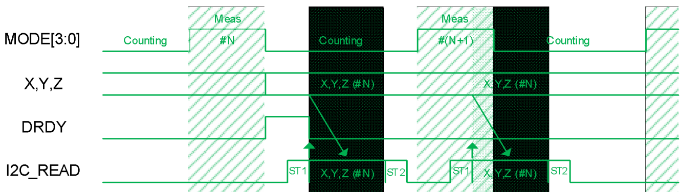
Figure 8: Data read start during measurement
