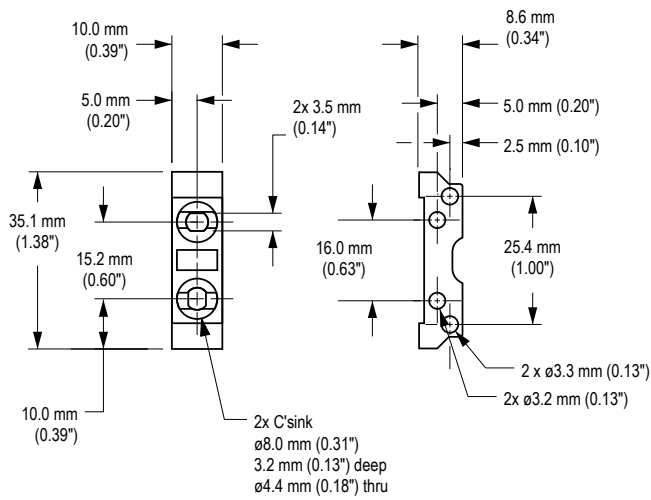
Figure 9. Included bracket dimensions
