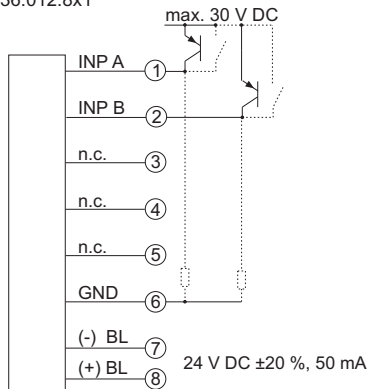
DC-Typ: 6.136.012.8x1
