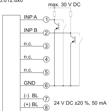
DC-Typ: 6.136.012.8x0
