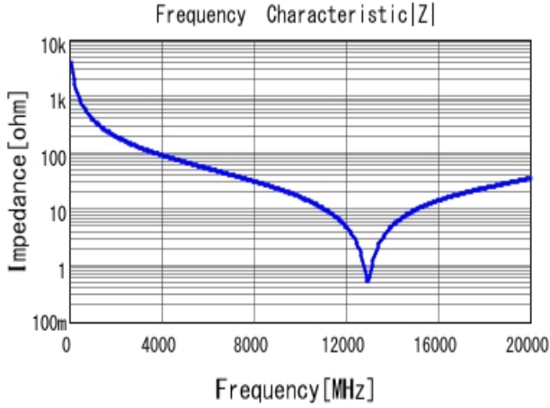
■ GJM1555C1HR40BB01 |Z| DC0V, 25degC
