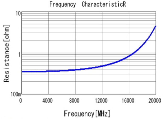
■ GJM1555C1HR40BB01 R DC0V, 25degC
