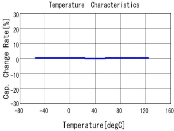
■ GRM1555C1H4R7WA01 C-Temp. capchange, DCOV, AC1Vrms
