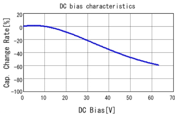
■ KCM55WR71J226MH01 C-DC bias capchange, 25.0degC, AC0.
