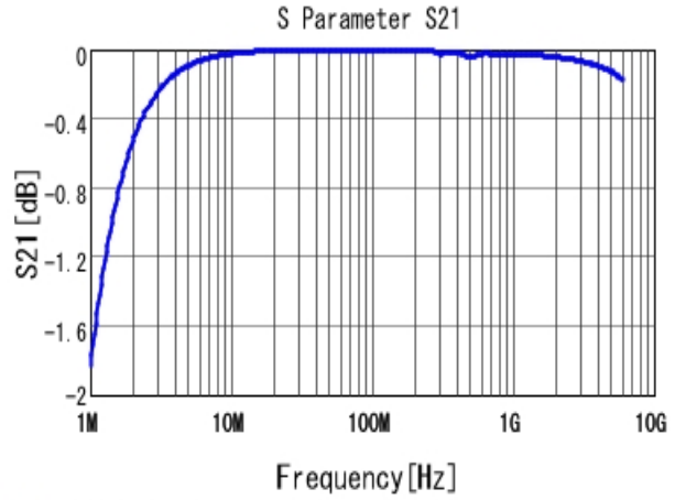
■ GRM1885C1H222JA01 S21 DCOV, 25degC
