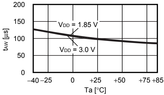
4.5 Awake mode time ( t_{AW} ) vs. Temperature ( T_a )
