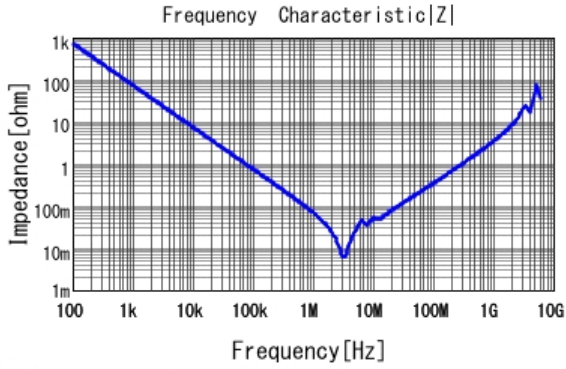
■ GRM43ER71H225KA01 |Z| DCOV, 25degC
