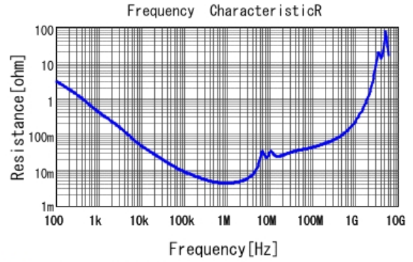
■ GRM43ER71H225KA01 R DCOV, 25degC
