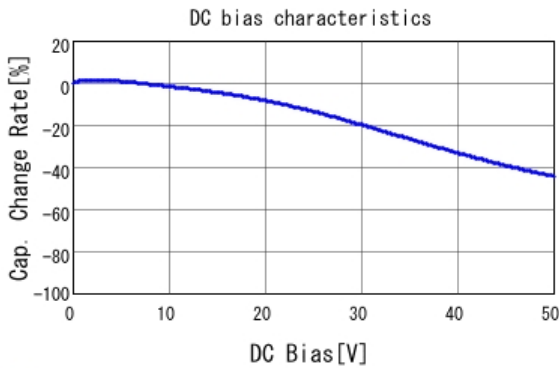
■ GRM43ER71H225KA01 C-DC bias capchange, 25.0degC, AC1.
