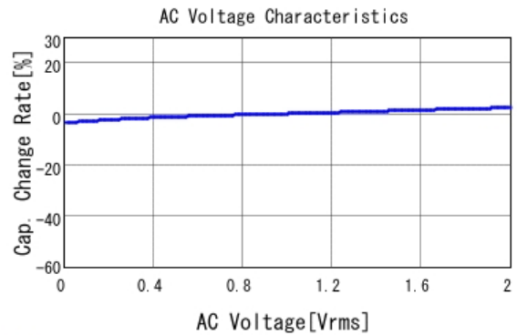
■ GRM43ER71H225KA01 C-AC Voltage capchange, DCOV, 25.0d
