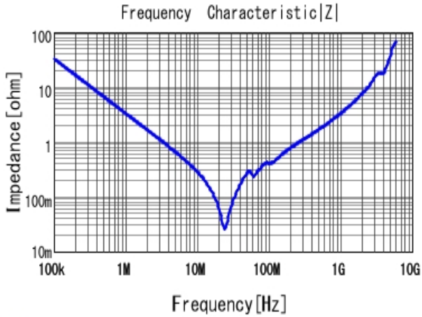
■ GRM43DR73A473KW01 |Z| DCOV, 25degC
