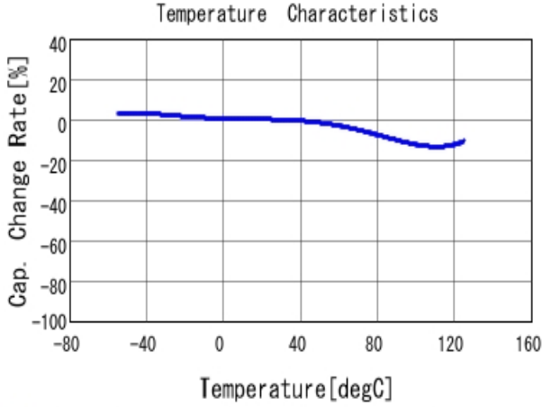
■ GRM43DR73A473KW01 C-Temp. capchange, DCOV, AC1Vrms
