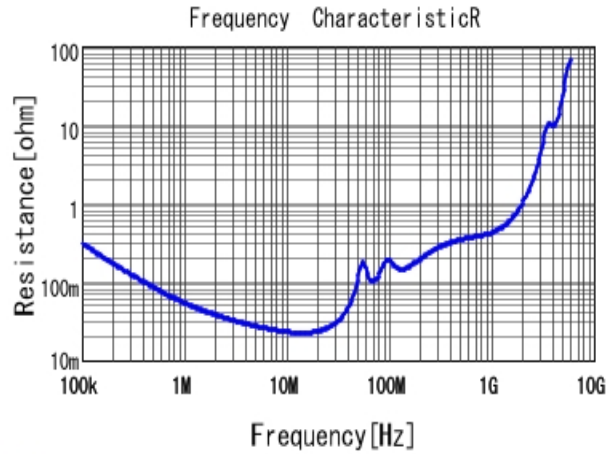
■ GRM43DR73A473KW01 R DCOV, 25degC
