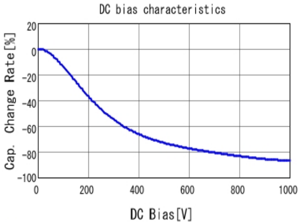
■ GRM43DR73A473KW01 C-DC bias capchange, 25.0degC, AC1V
