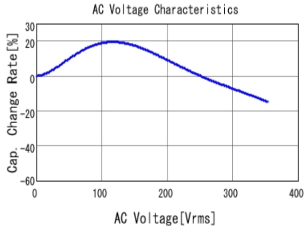
■ GRM43DR73A473KW01 C-AC Voltage capchange, DCOV, 25.0d
