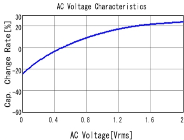
■ GRM32EC81C476ME15 C-AC Voltage capchange, DCOV, 25.0d
