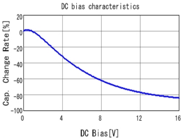
■ GRM32EC81C476ME15 C-DC bias capchange, 25.0degC, ACO.
