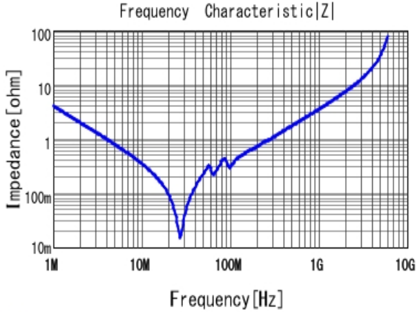
■ GRM31M5C1H393JA01 |Z| DCOV, 25degC
