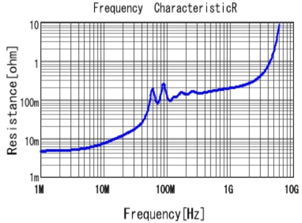
■ GRM31M5C1H393JA01 R DCOV, 25degC
