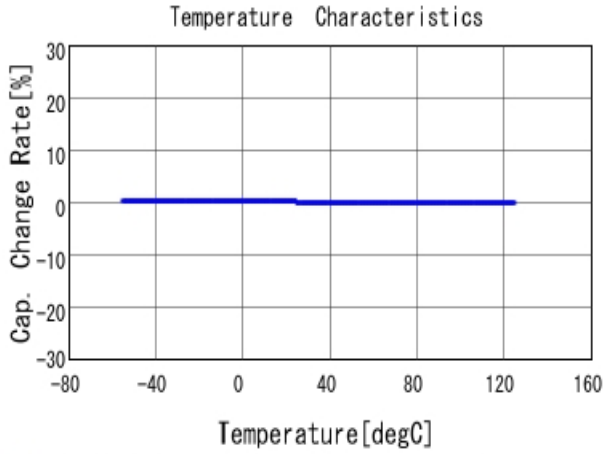
■ GRM31M5C1H393JA01 C-Temp. capchange, DCOV, AC1Vrms
