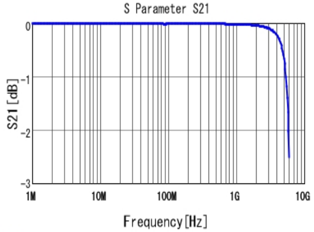
■ GRM31M5C1H393JA01 S21 DCOV, 25degC
