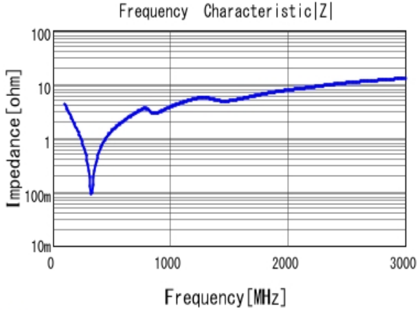
■ GRM31A7U3A331JW31 |Z| DCOV, 25degC
