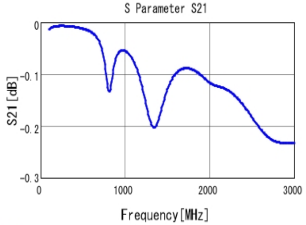
■ GRM31A7U3A331JW31 S21 DCOV, 25degC
