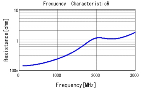
■ GRM31A7U2J101JW31 R DCOV, 25degC
