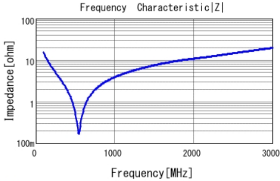
■ GRM31A7U2J101JW31 |Z| DCOV, 25degC
